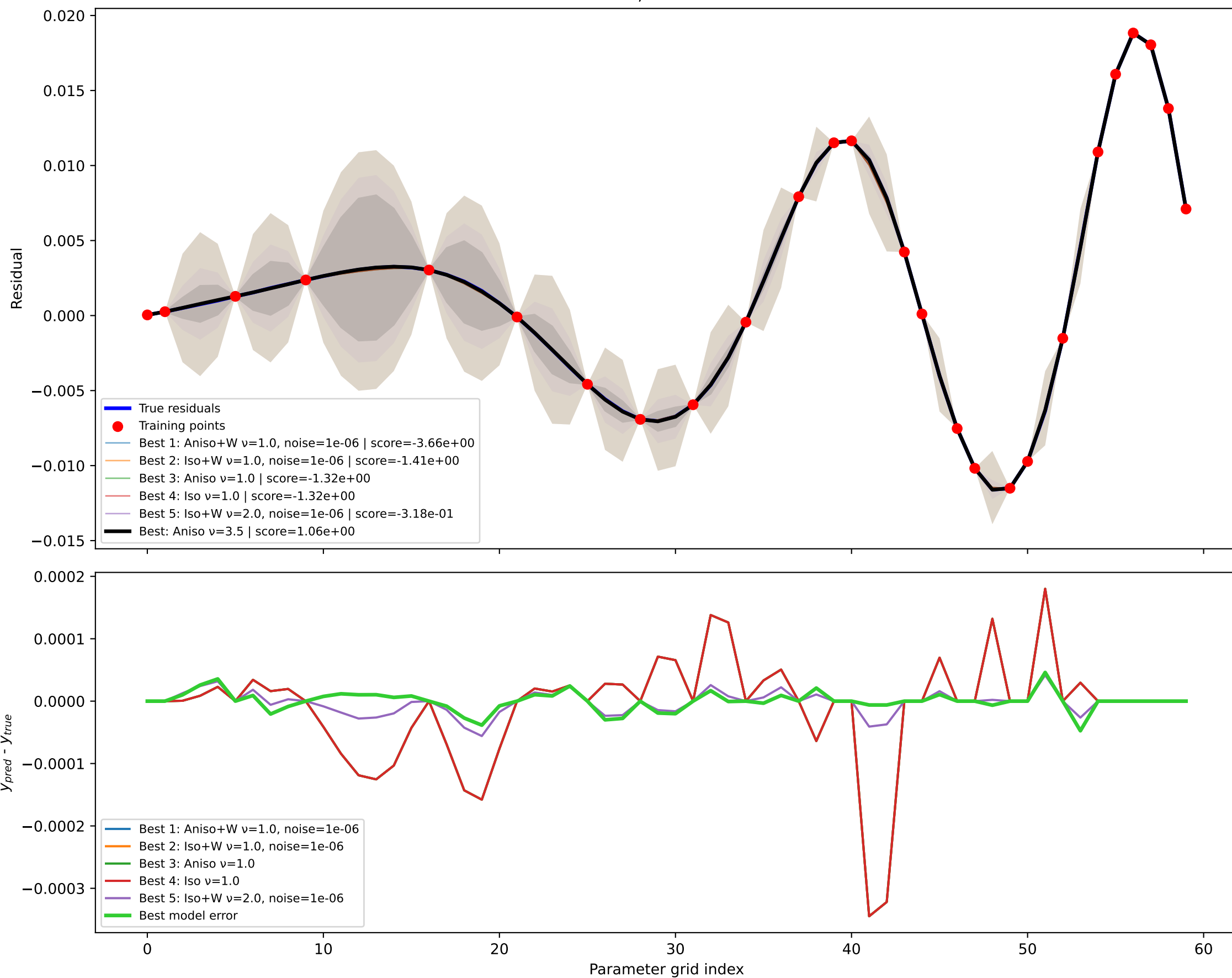
GPR kernel comparison node=22 RMSE=1.532e-05, train RMSE=9.046e-12
